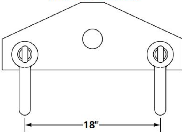
T46HD Ground Release II Spreader Beam with Twin Shackles
