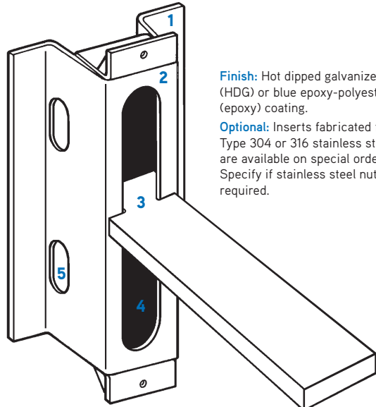
P31 Corewall Strap Type Slotted Insert
