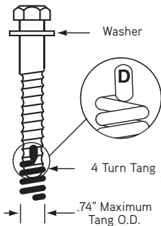
T13 Coil Anchor Bolt Patent #5,006,023 3/4" Dia. x 4-1/2" Long
