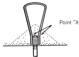
Dotted line indicates line of probable concrete failure Point "X" - point of possible strut fracture.
