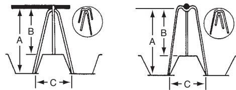
CHC-Continuous High Chairs for Metal Decking
