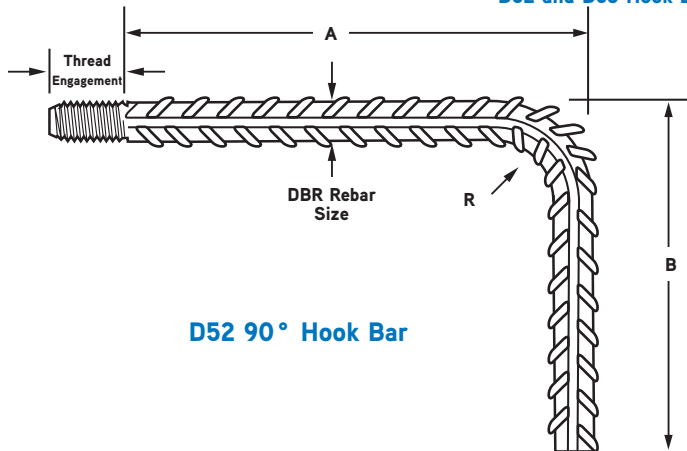
D52 and D53 Hook Bar Selection Chart
