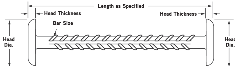
D158E/D158J Double End Anchor (Forged Heads)
