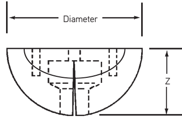
Swift Lift Round Recess Plug
