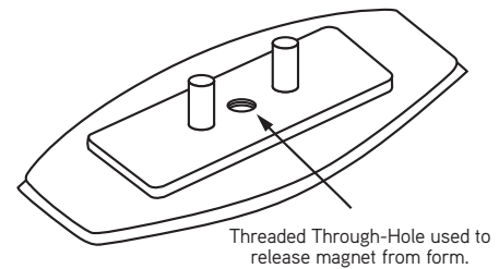
P76M Utility Anchor Magnetic Setting Plate
