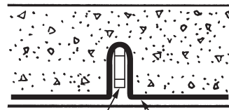
Erection Anchor Shear Bar
