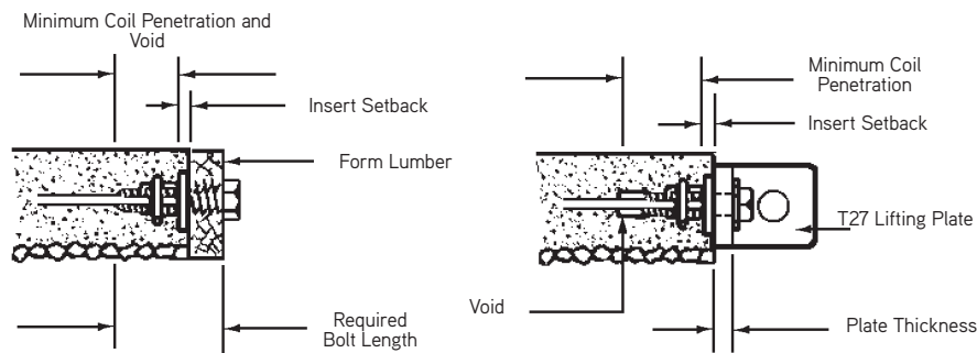
Setting Bolt
