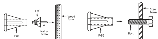
P86 Form Installation Using F74 Threaded Plastic Plug
