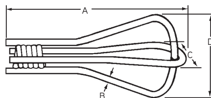
B33 Double Flared Coil Loop Insert
