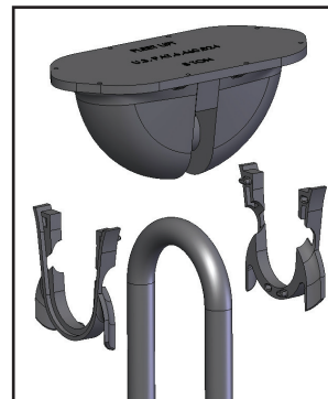
P99D assembly view
