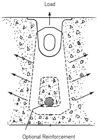
Optional Reinforcement
