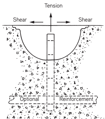
Resists Tension and Shear Loads
