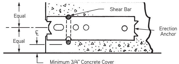
Section View
