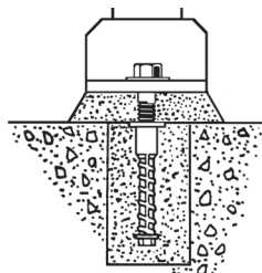
Core and Grout Application
