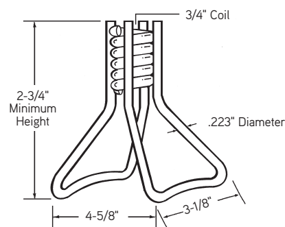
F47 Double Flared Loop Insert
