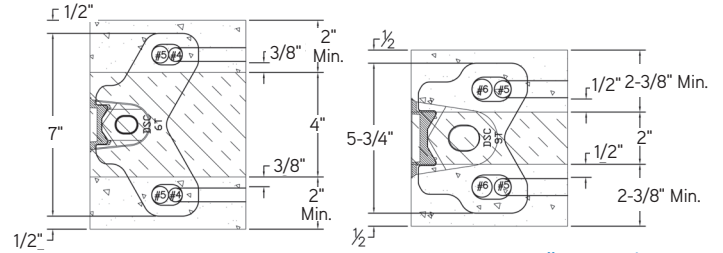
6-Ton P92SF for 4" Insulation 9-Ton P92SF for 2" Insulation
