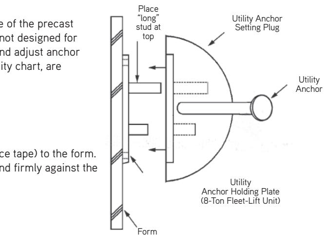
In-Form Setting
