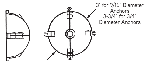
P54 Swift Lift Recess Plug
