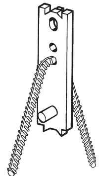
Typical P92P Fleet-Lift Erection Anchor Shear Plate/Tension Bar Application
