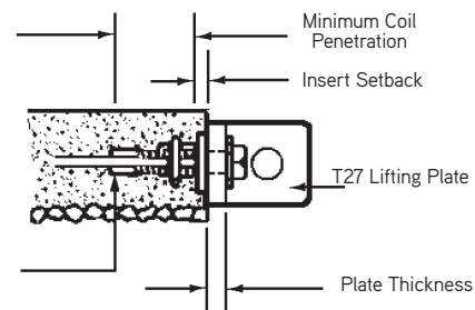
Lifting Bolt
