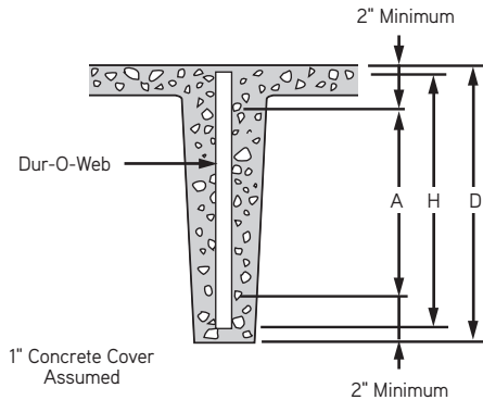
Double Tee
