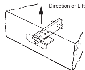
Typical P92P Fleet-Lift Erection Anchor with Shear Plate Application
