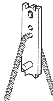
Typical P92P Fleet-Lift Erection Anchor Shear Plate/Tension Bar Application
