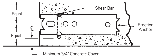
Section View
