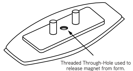
P76M Utility Anchor Magnetic Setting Plate
