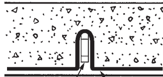
Erection Anchor Shear Bar
