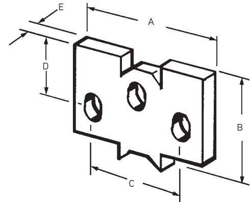
P92S Fleet-Lift Sandwich Panel Erection Anchor
