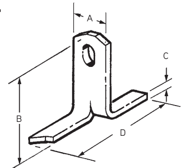
P95F Fleet-Lift Flat Foot Anchor
