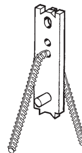
Typical P92 Fleet-Lift Erection Anchor/Tension Bar Application
