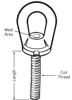
F49 Eye Bolt
