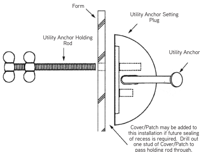
Through-Form Setting
