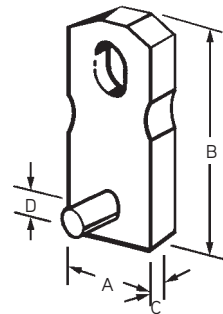
P94 Fleet-Lift T-Anchor 4-ton
