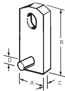
P94 Fleet-Lift T-Anchor 2, 6 and 8-ton
