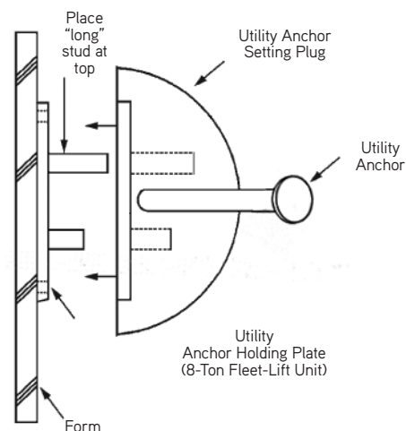
In-Form Setting
