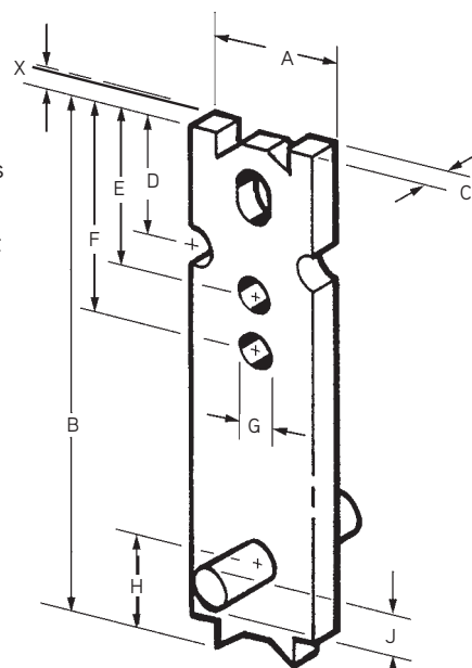
P92 Fleet-Lift Erection Anchor
