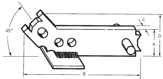
P92AH Fleet-Lift Erection Anchor with 45° Head with Shear Plate
