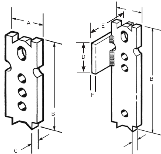
P92H Fleet-Lift Two-Hole Erection Anchor (Tension Loadings ONLY)
