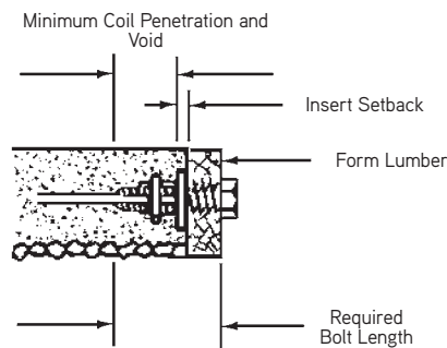
Setting Bolt
