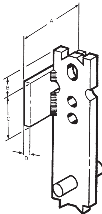
P92P Fleet-Lift Erection Anchor with Shear Plate
