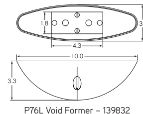
P76L Void Former - 139832
