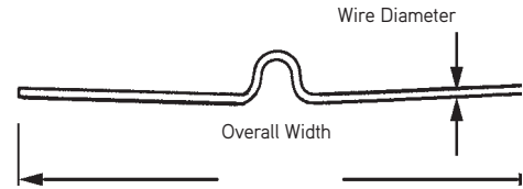
P59 Swift Lift Smooth Wire Shear Bar 2-Ton and 4-Ton When used with P54 Throw-Away Recess Plug
