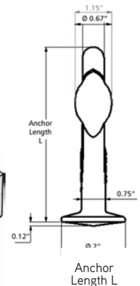
P76L Void Former - 139832
