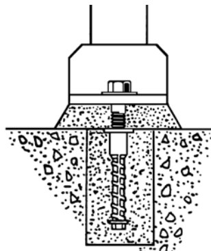
Core and Grout Application
