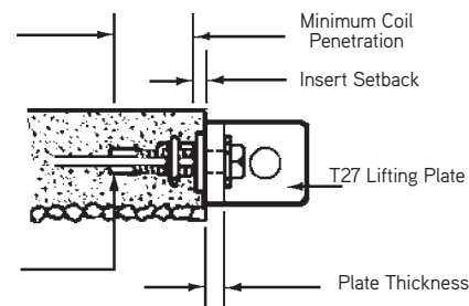
Lifting Bolt
