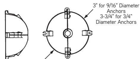
P54 Swift Lift Recess Plug
