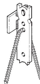
Typical P92HP Fleet-Lift Two-Hole Erection Anchor with Shear Plate/Tension Bar Application
