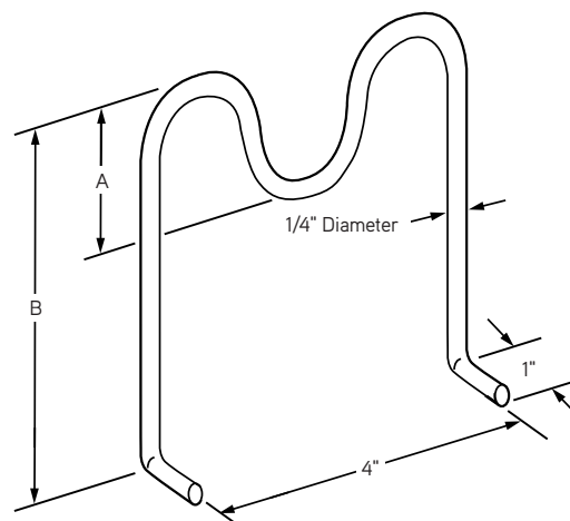
P37 "M" Anchor Shear Connector
