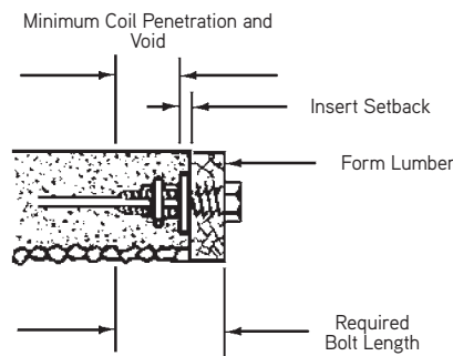
Setting Bolt
