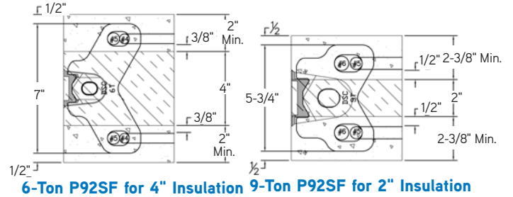
6-Ton P92SF for 4" Insulation 9-Ton P92SF for 2" Insulation
