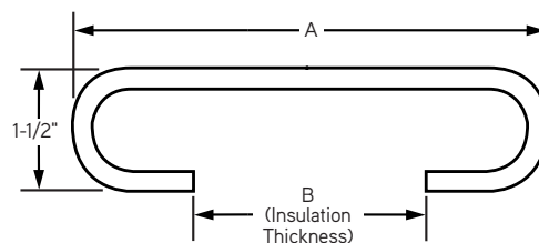
P9 Precast Sandwich Panel Tie
