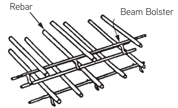
Beam Bolster
