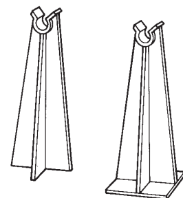
Snap-On Paving Chairs
