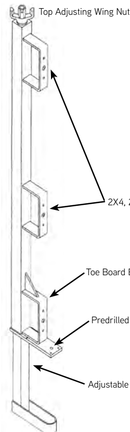
A93 Sure Guard Rail Post System
