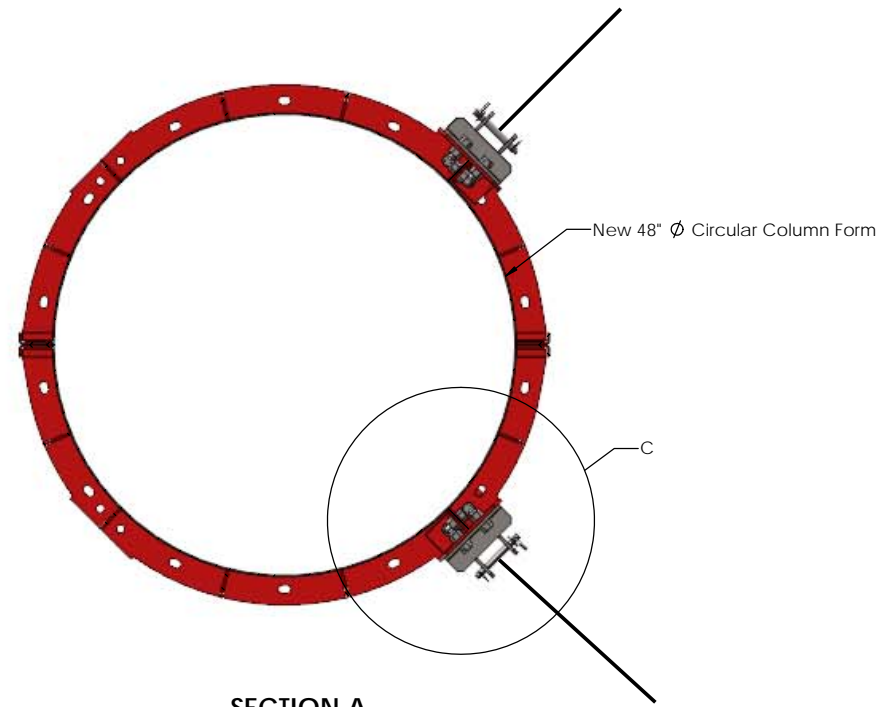
SECTION A
