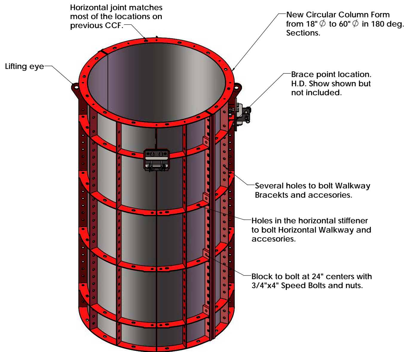
New Circular Column Form in 180 Deg. Sections from 18" \phi to 60" \phi CCF. Allowable Pour Pressure is 3,000 psf.
