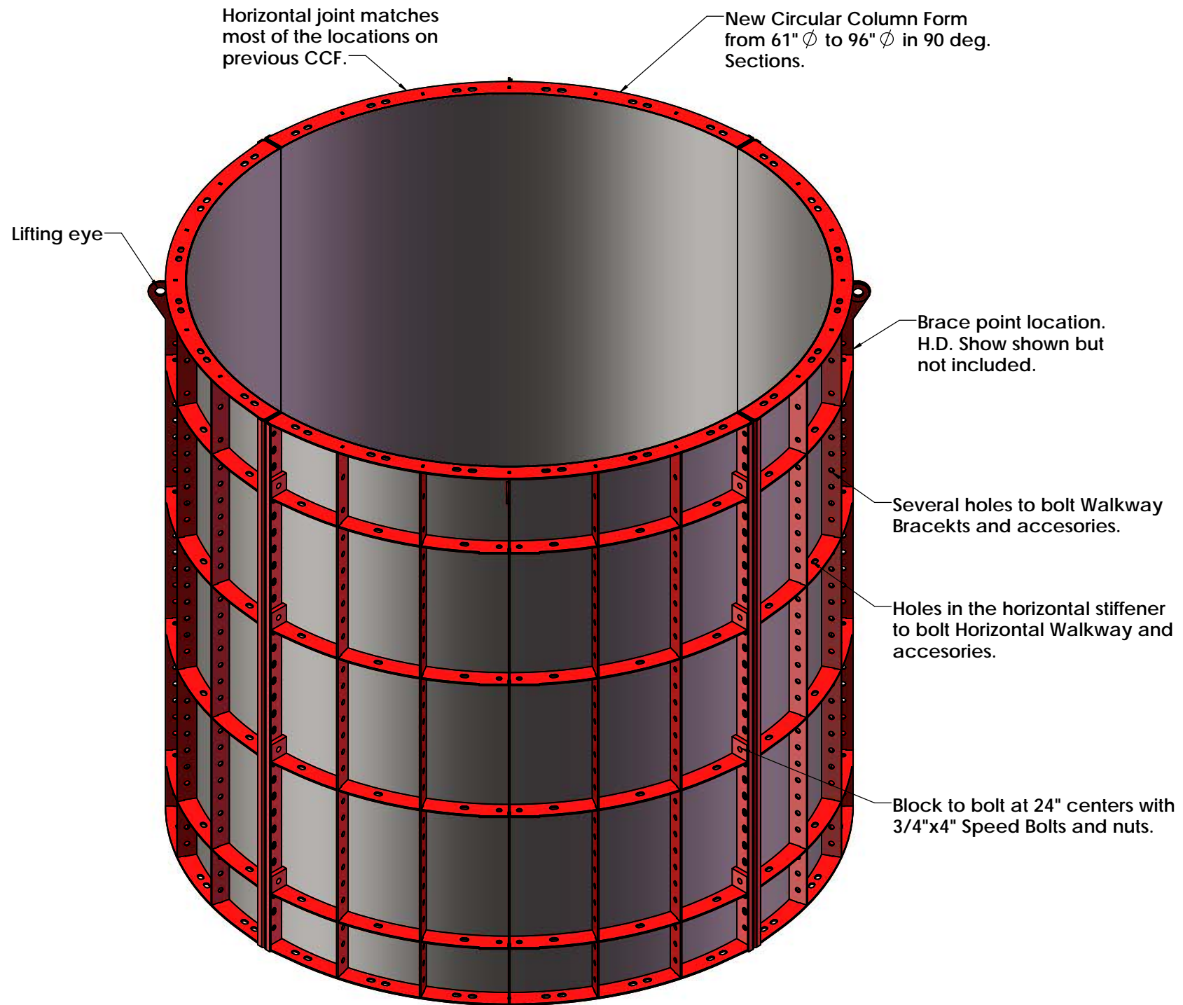
New Circular Column Form in 90 Deg. Sections from 61" \phi to 96" \phi CCF. Allowable Pour Pressure is 2,000 psf.
