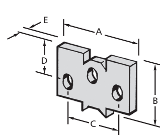
P92S SANDWICH PANEL ERECTION ANCHOR
