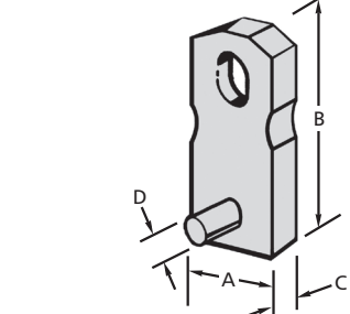
P92FEWDP FORGED ERECTION ANCHOR WITH PRIMARY AND SECONDARY SHEAR NEW GENERATION
