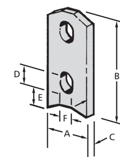
P96 TWO-HOLE ANCHOR
