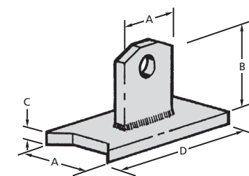
P95P PLATE ANCHOR
