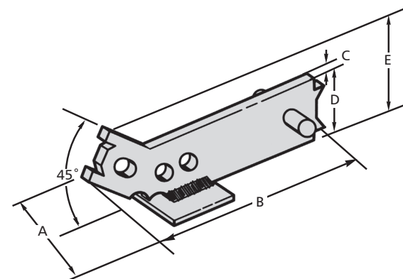
P92AH ERECTION ANCHOR WITH 45° HEAD WITH SHEAR PLATE
