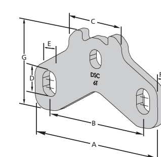
P92SF FORGED SANDWICH PANEL ERECTION ANCHOR NEW GENERATION
