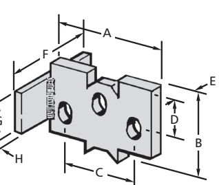
P92SP SANDWICH PANEL ERECTION ANCHOR WITH SHEAR PLATE
