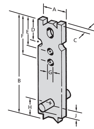
P92 ERECTION ANCHOR
