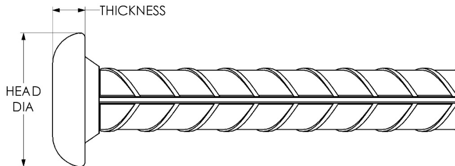
FIGURE 4 – D155 Forged End Anchors
