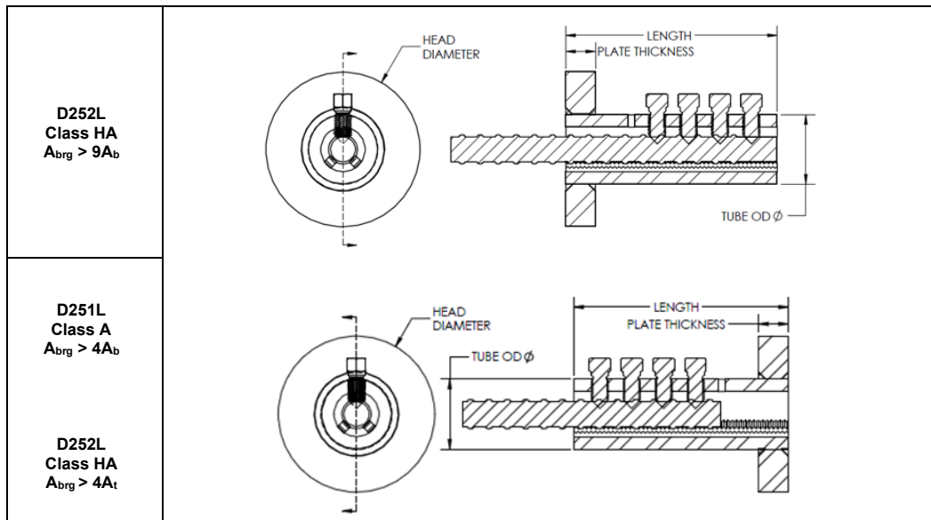
FIGURE 2 – Bar-Lock End Anchor
