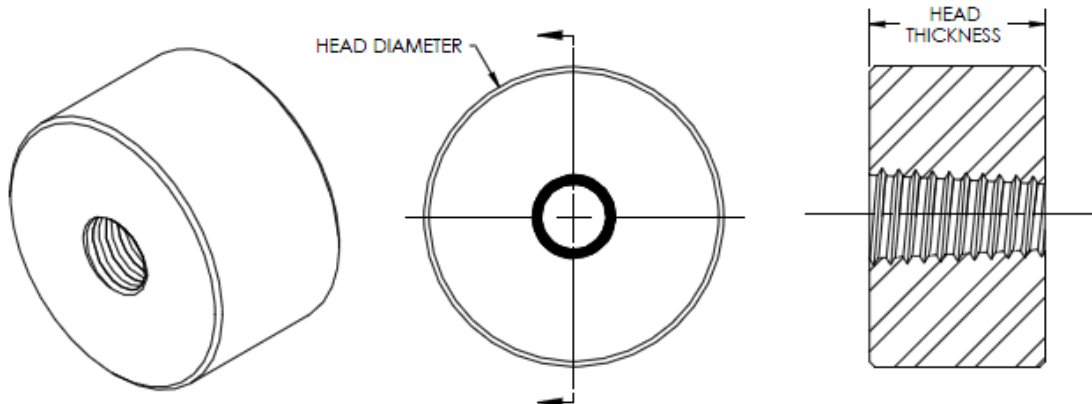
FIGURE 1 – D350 / D351 End Anchor
