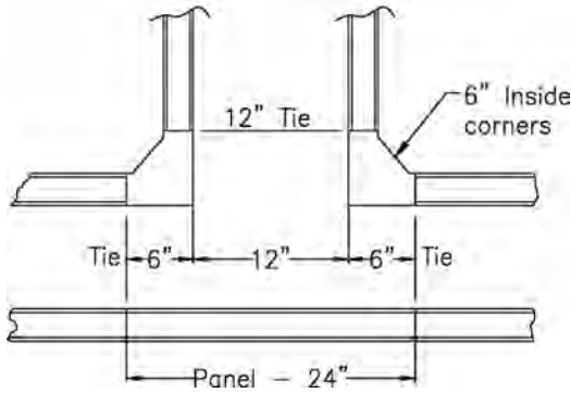
Typical Form and Tie Configuration for Intersecting Walls 12" Thick or Less
