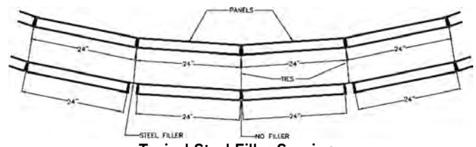
Typical Steel Filler Spacing
