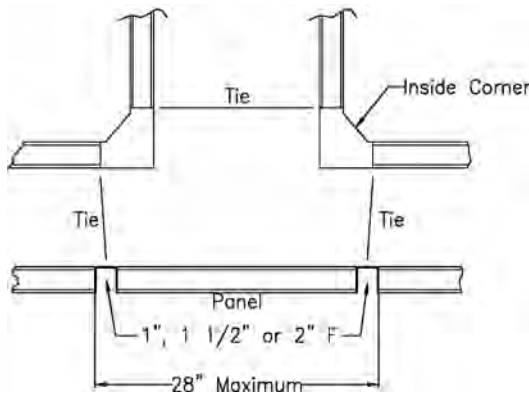
Typical Form and Tie Configuration for Intersecting Walls 13" to 16"
