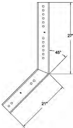
5" x 45° Splice Channel
