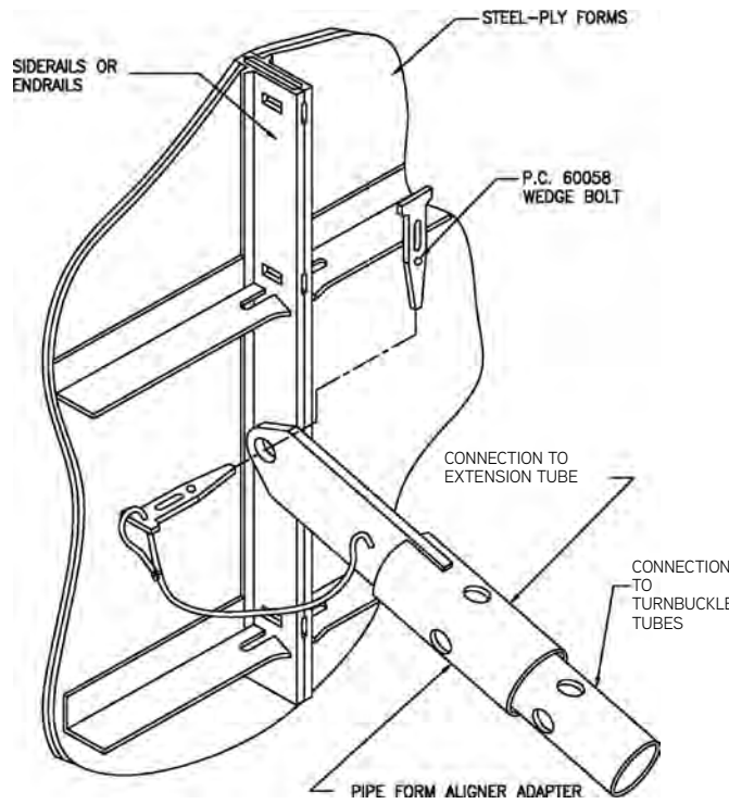
Pipe Form Aligner Attachment to Steel-Ply
