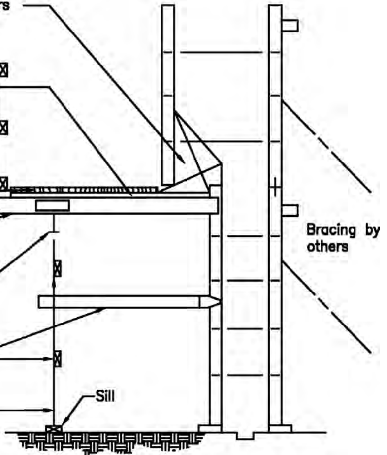
Typical Haunch Support Bracket Application
