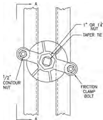
Cast Bearing Washer and Taper Tie Detail
