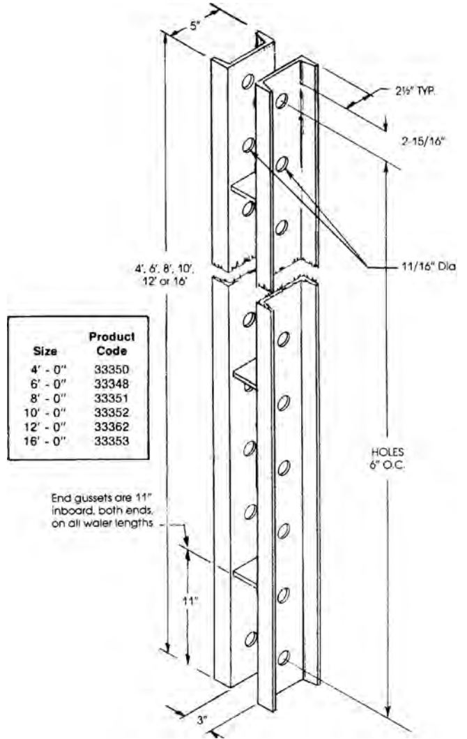
5" Walers
