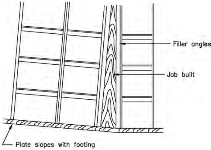
Typical Sloped Transition to Plumb Forms
