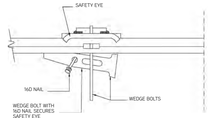
Safety Eye Installation
