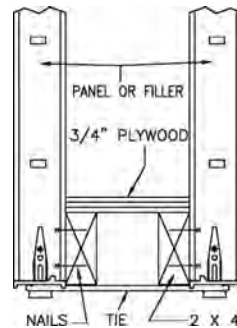
Lumber Bulkhead
