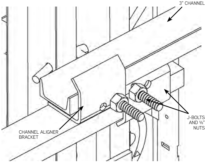
3" Channel Strongback Connection
