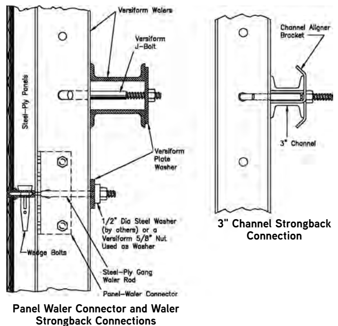
Section View
