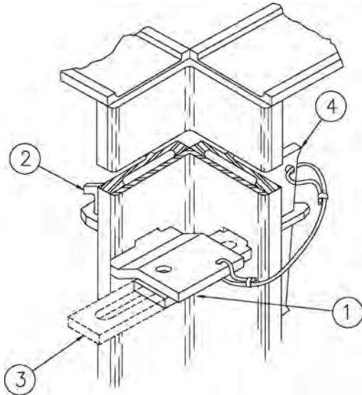
Quick Column Hardware Installation
