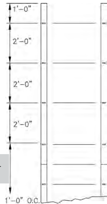
Tie Spacings Walls Taller Than 8' 6,000 lb Ultimate Tie Capacity
