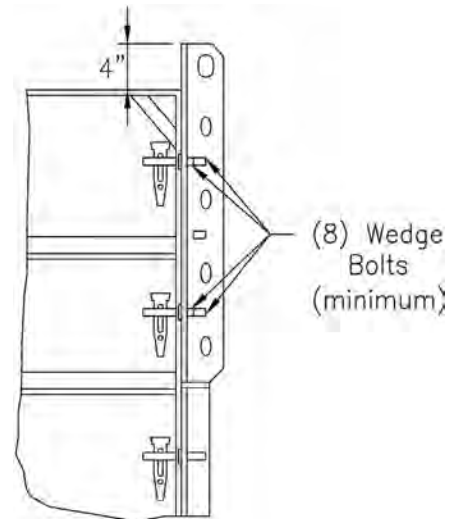
Column Lift Corner Installation
