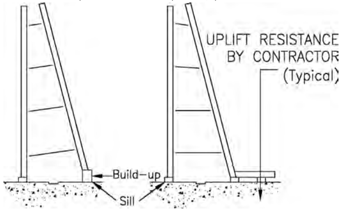
Typical Battered Wall Configuration
