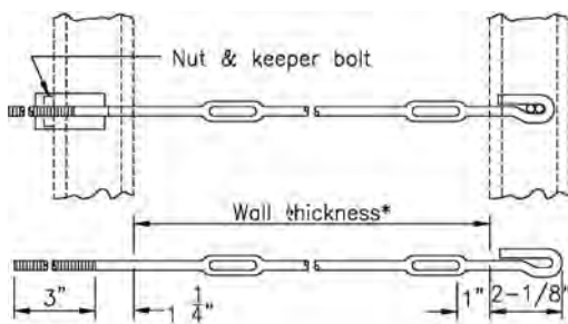
Single End Threaded Tie
