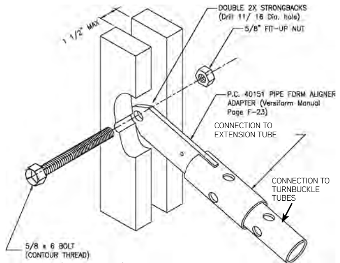
Pipe Form Aligner Attachment to Strongbacks
