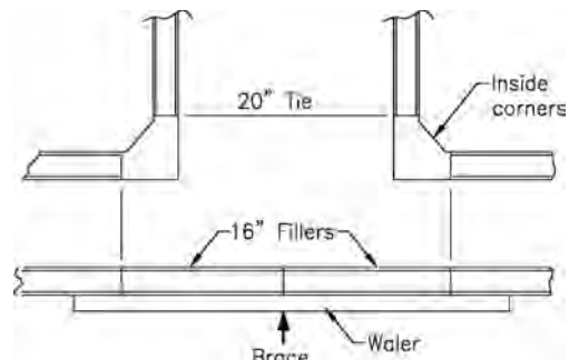
Application Using Walers and Braces for Intersecting Walls over 16"
