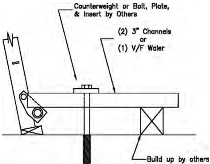
Battered Wall Tie Down
