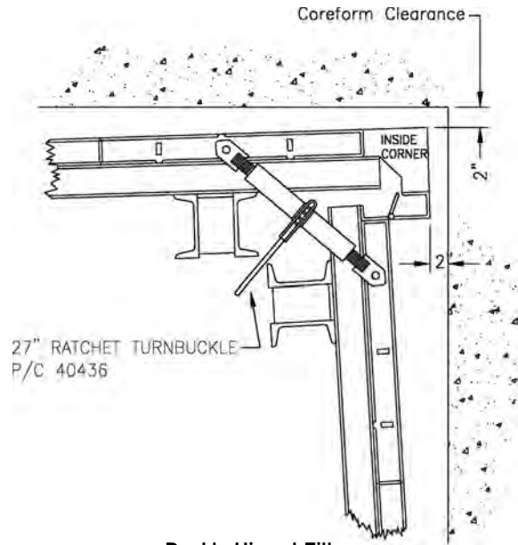
Double Hinged Filler (in fold position)
