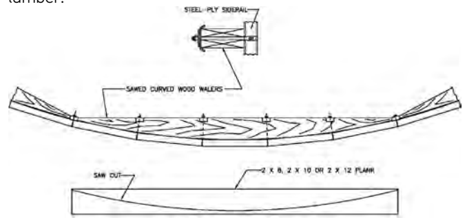
Typical Attachment of Lumber Waler Cut to Curve
