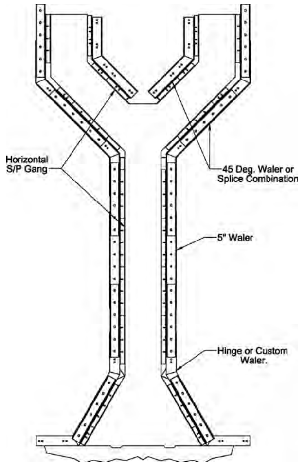
Typical Form Configuration for “Y” Wall
