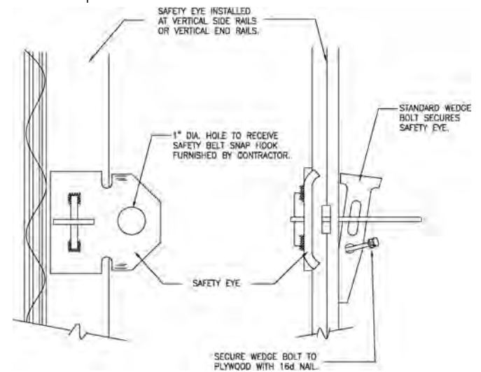
Safety Eye Installation
