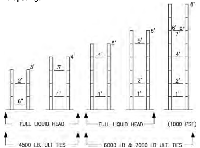
Tie Spacings Walls 8' Tall or Less
