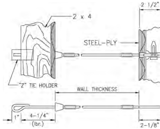
#2A Cone Tie
