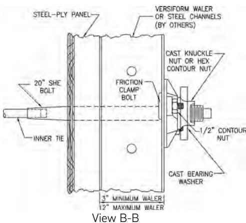
Cast Bearing Washer and She-Bolt Detail
