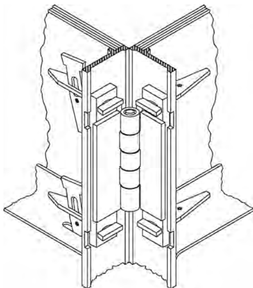
Column Hinge Installation
