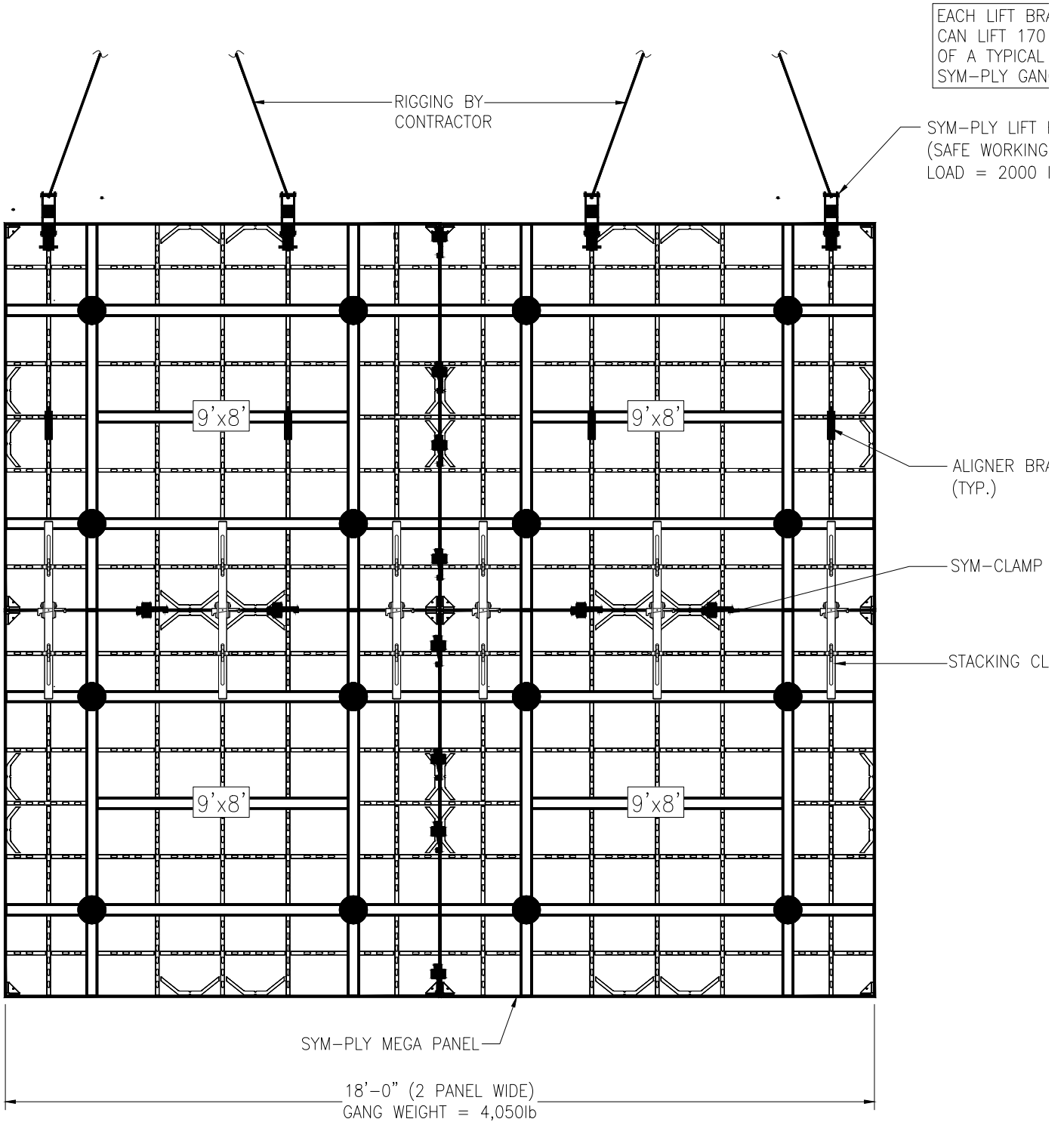
GANG - 2 Panels Wide x 2 Panels Tall - Part#: F56000 (9' Wide x 8' Tall)
