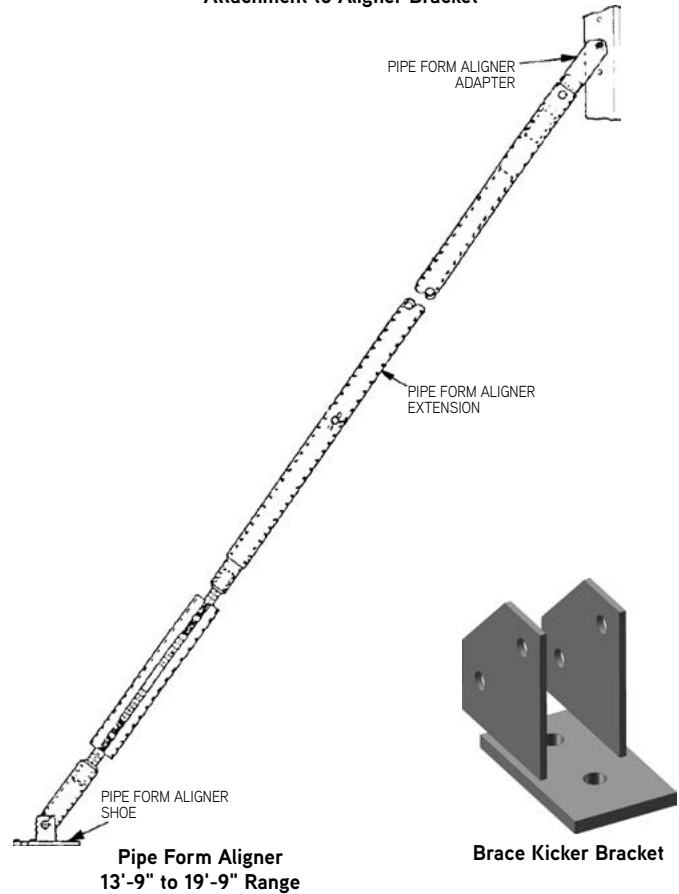
Attachment to Aligner Bracket
