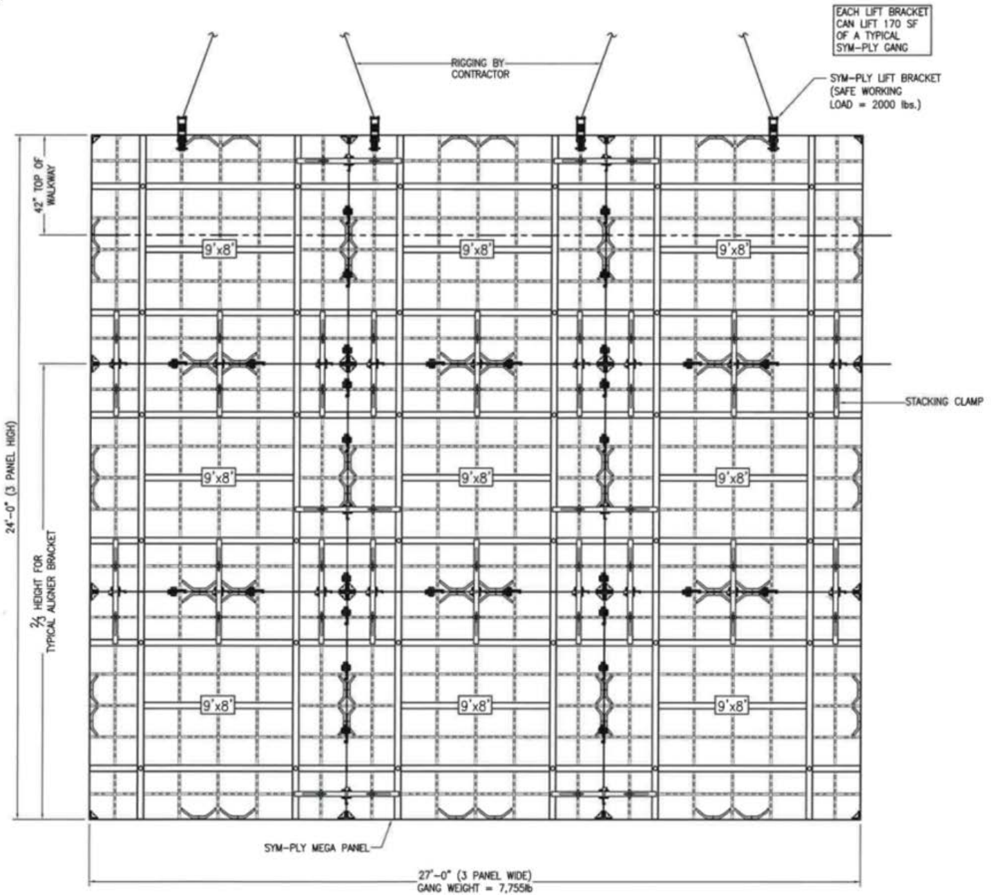
3 (9x8 Panels) Wide x 3 (9x8 Panels) Tall
