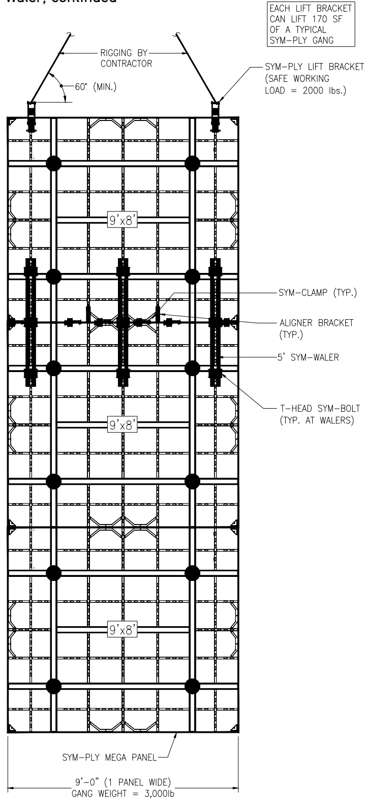
GANG - 1 Panel Wide x 3 Panels Tall - Part#: F56000 (9' Wide x 8' Tall)
