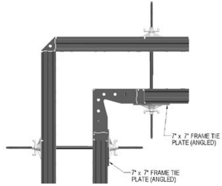
90° Corner with Fillers at Inside Corner
