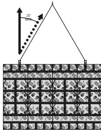
2,000 lbs. at 5 to 1 Safety Factor
