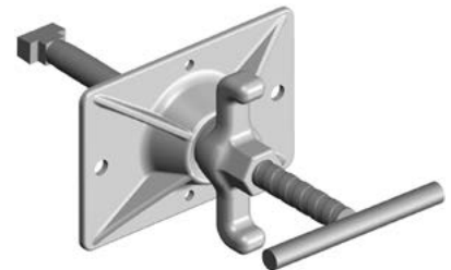
T-Head Sym-Bolt Assembly Long
