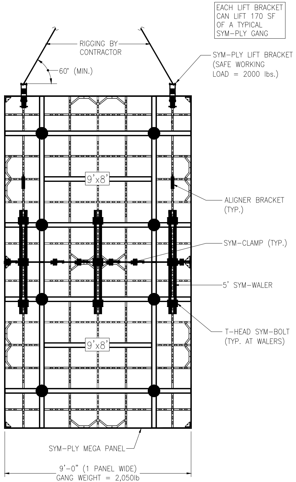
GANG - 1 Panel Wide x 2 Panels Tall - Part#: F56000 (9' Wide x 8' Tall)
