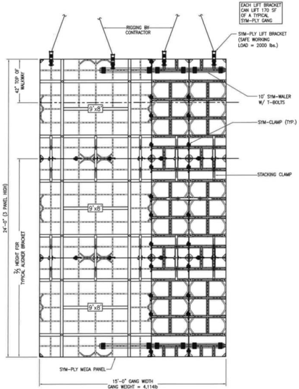
Example Gang Attachment of 9x8 Panel to 3x8 Panel
