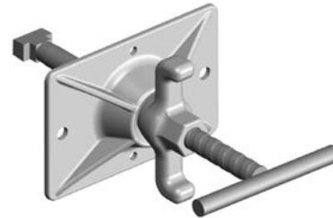
T-Head Sym-Bolt Assembly
