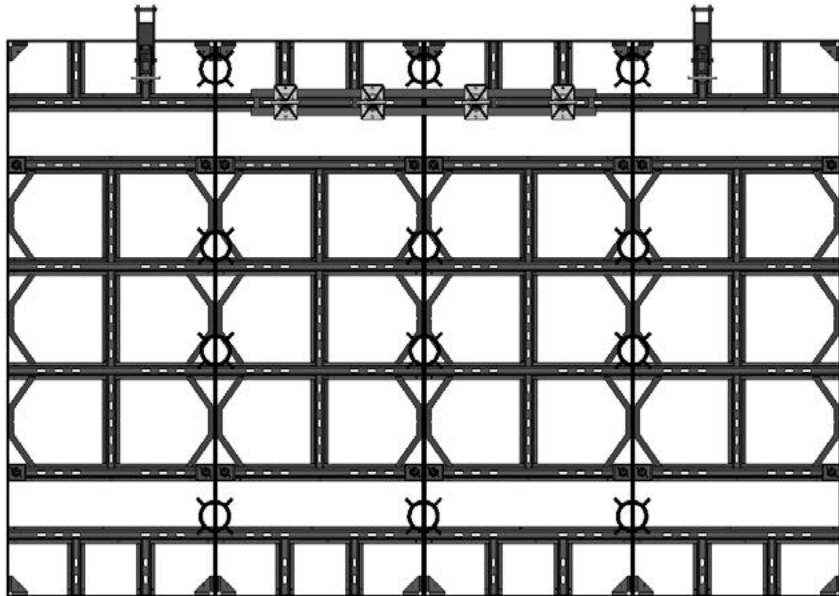
GANG – 3'-0" Wide x 8'-0" High x 4 Panels Wide
