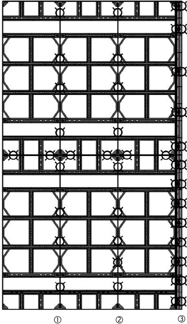
Corner and Bulkhead Clamp Spacing (for Panel Widths of 3' and 2'-6")
