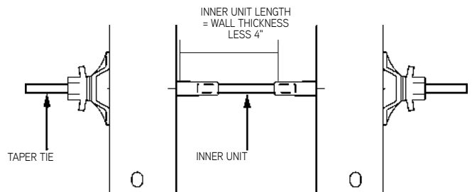
Typical She-Bolt Application
