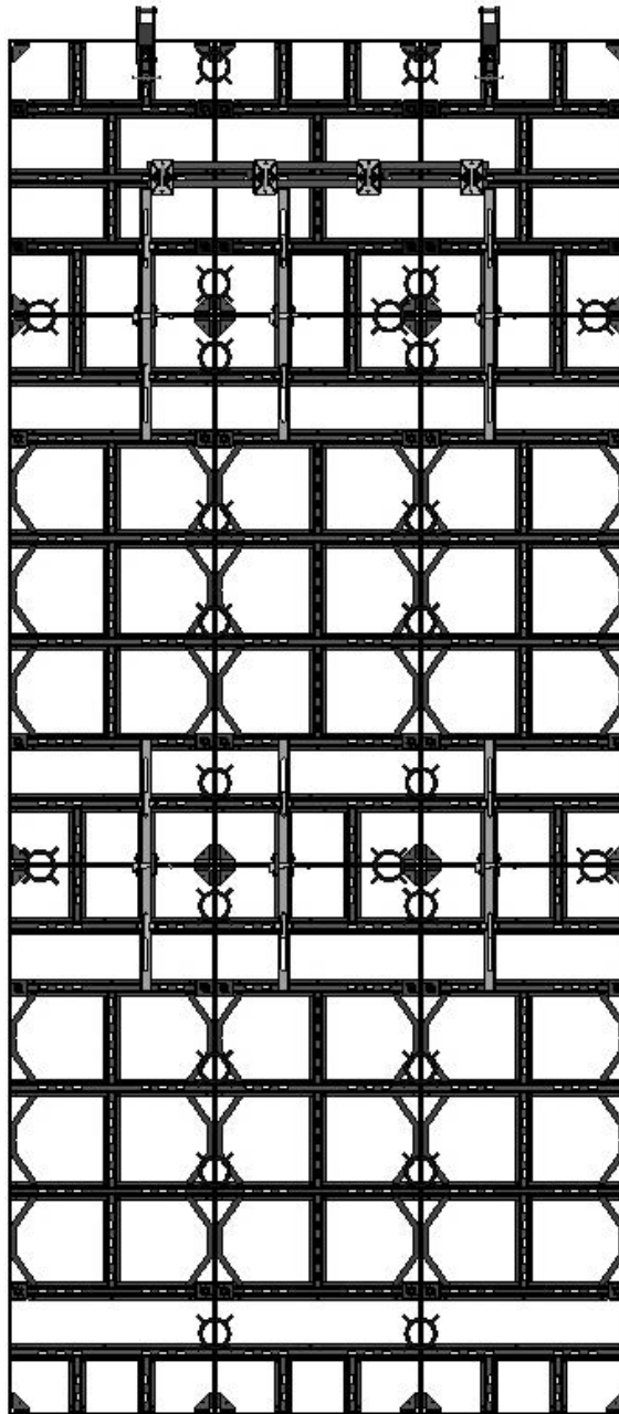
GANG – 3'-0" Wide x 8'-0" High + 8'-0" High + 4'-0" High x 3 Panels Wide
