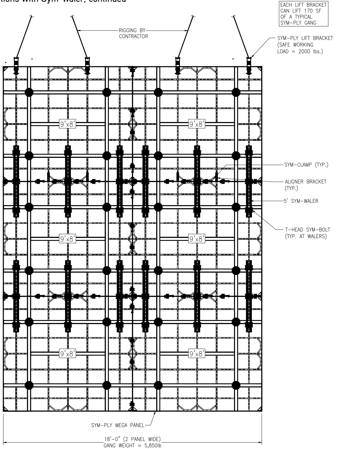
GANG - 2 Panels Wide x 3 Panels Tall - Part#: F56000 (9' Wide x 8' Tall)
