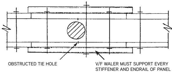
Using a Versiform Waler to Avoid Obstructions
