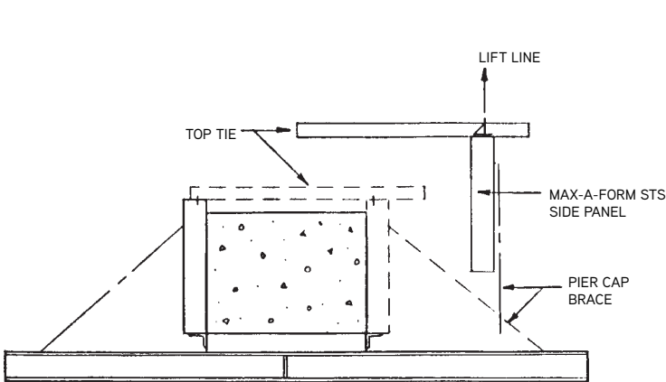
"I" Section Pick ( "L" Section supported by Screw Jacks )
