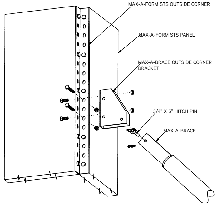
Max-A-Brace Outside Corner Bracket Connection to Max-A-Form STS Column Form
