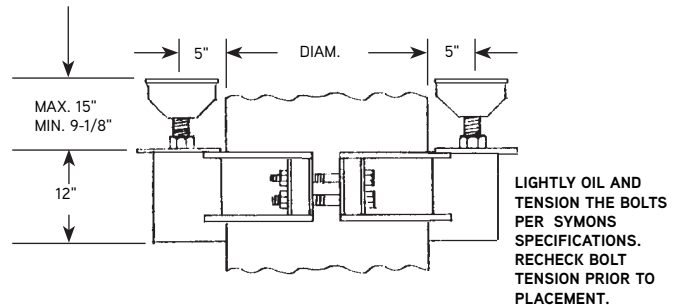
Circular Friction Collar
