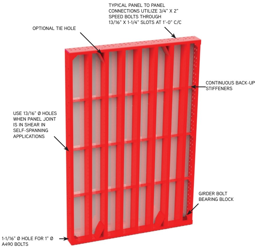
Typical Max-A-Form STS Panel
