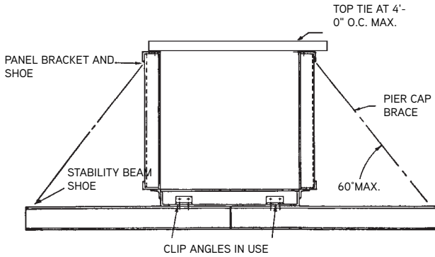
Stability Beam attached to Soffit
