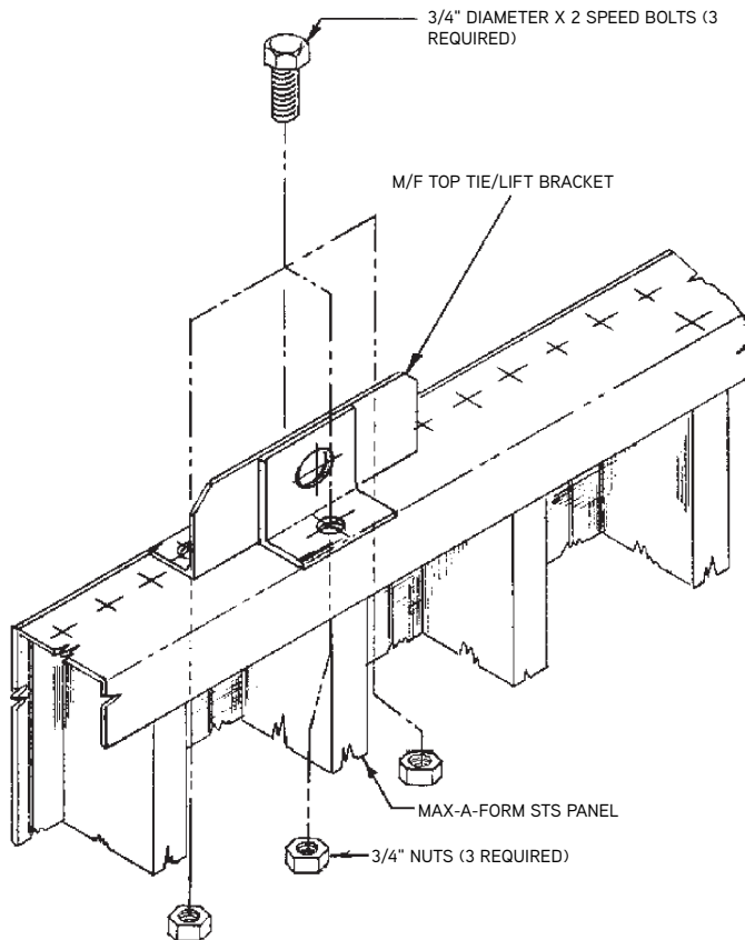
Max-A-Form STS Top Tie/Lift Bracket Installation
