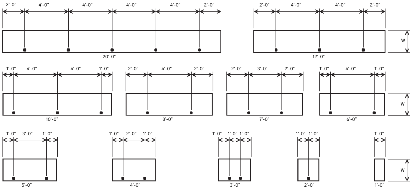
Tie Locations for Max-A-Form STS Panels
