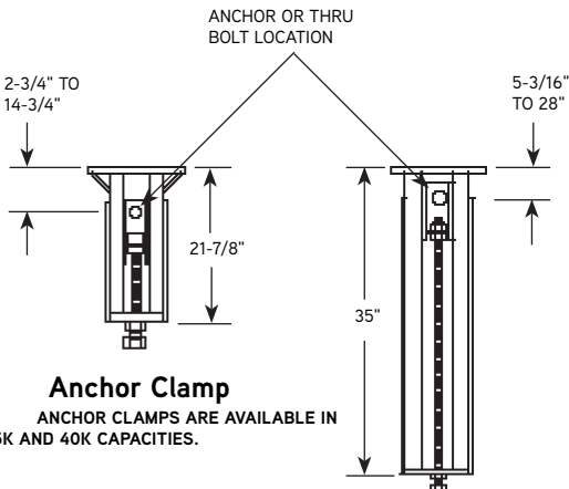
Adjustable Anchor Clamp
