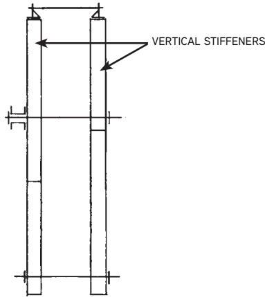
Using a Versiform Waler to Correct Vertical Misalignment
