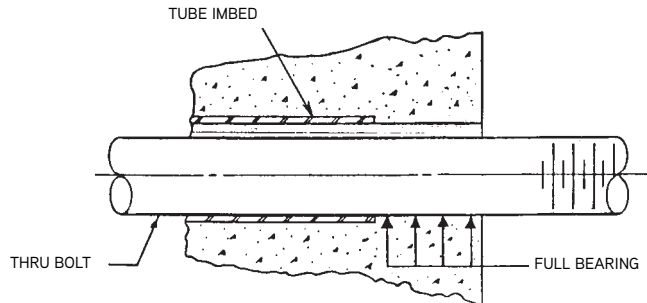
Section - Thru-Bolt Inserted
