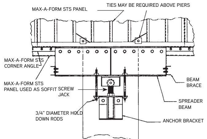
Section at Pier
