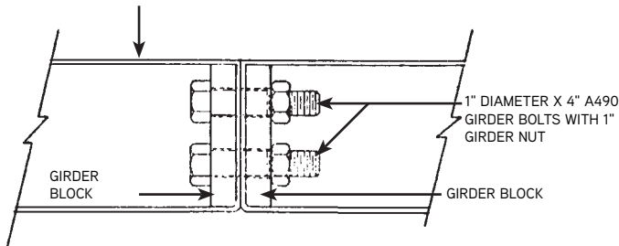
TYPICAL PANEL CORNER SHOWING GIRDER BOLT CONNECTION WITH TWO (2) 1" DIAMETER A490 GIRDER BOLTS
