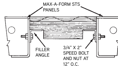
3/4" Plywood with 2" x 4" wood backing
