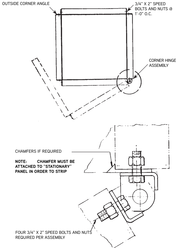
Detail at Hinge
