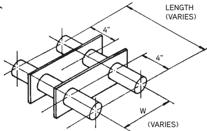
70 and 140 KIP Imbeds
