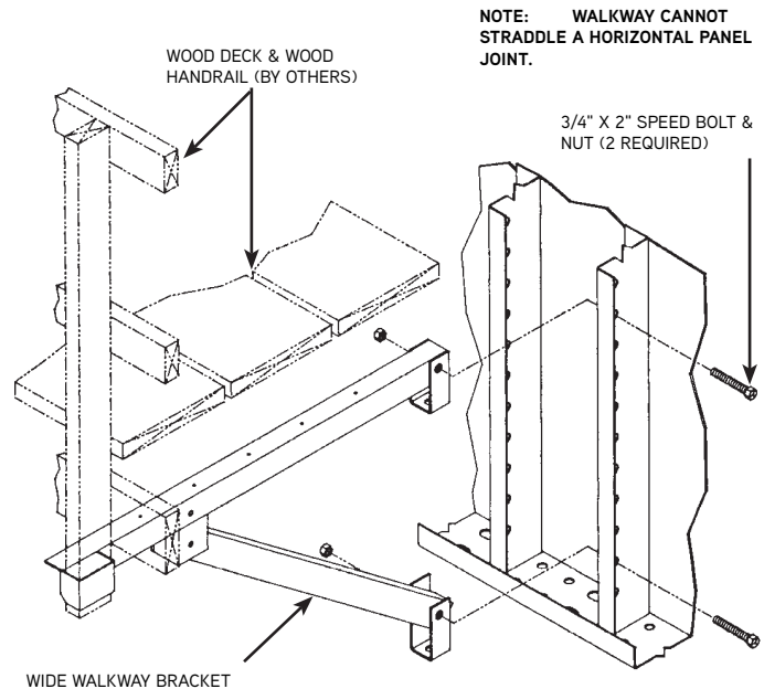
Wide Walkway Bracket Installation for Vertical Stiffeners
