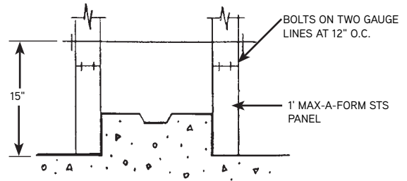
Raised Form
