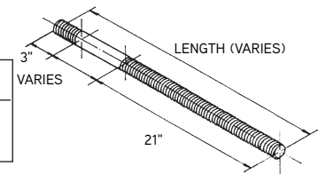
Thru-Bolts with Nuts
