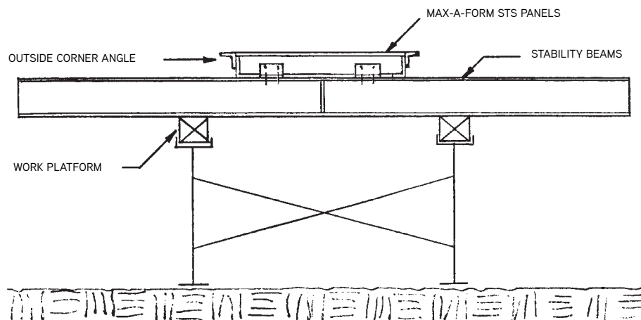
Alternate Method
