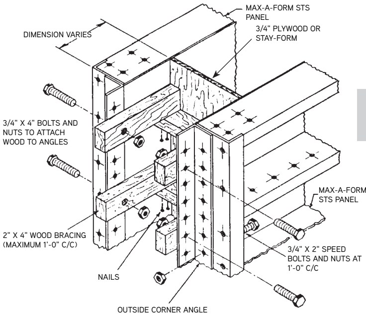
Outside Corner Angles used for End Bulkheads Maximum width 2'-0"
