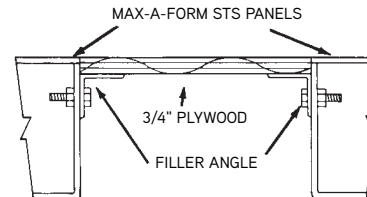
3/4" Plywood without 2" x 4" wood backing
