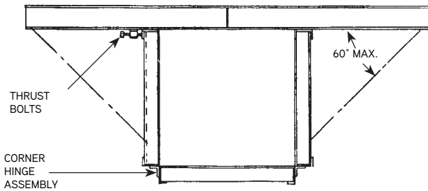
Stability Beam attached to Side Panels
