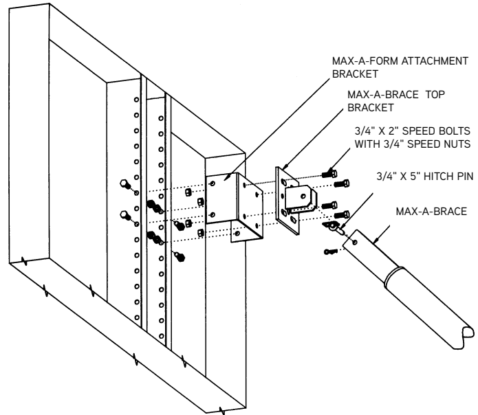
Max-A-Form STS Attachment Bracket and Max-A-Brace Top bracket connection to Max-A-Form STS panel with vertical stiffeners
