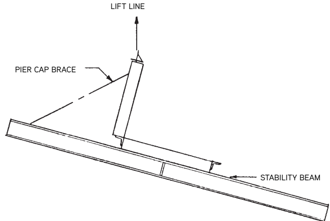
"L" Section - 2nd Pick
