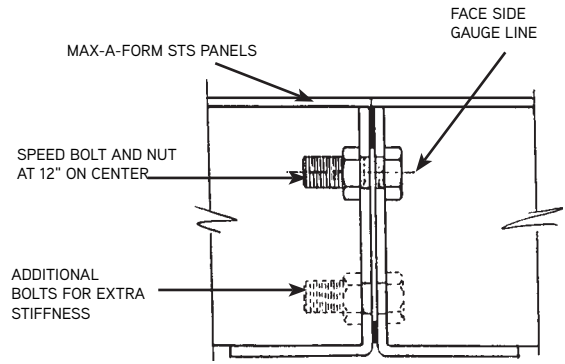
Max-A-Form STS Panel-To-Panel Bolt Connection
