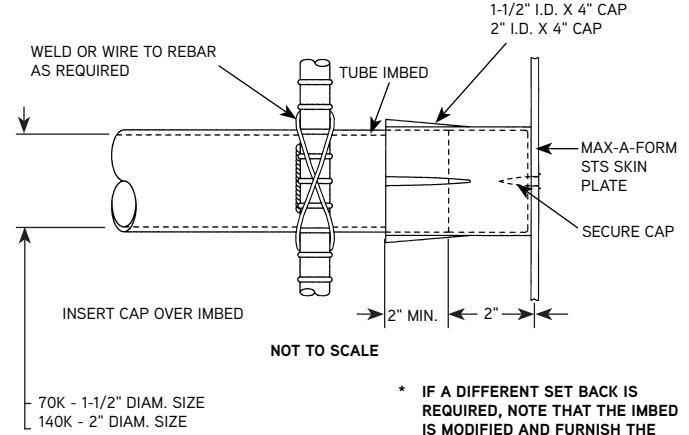
Section Imbed and Cap During Pour
