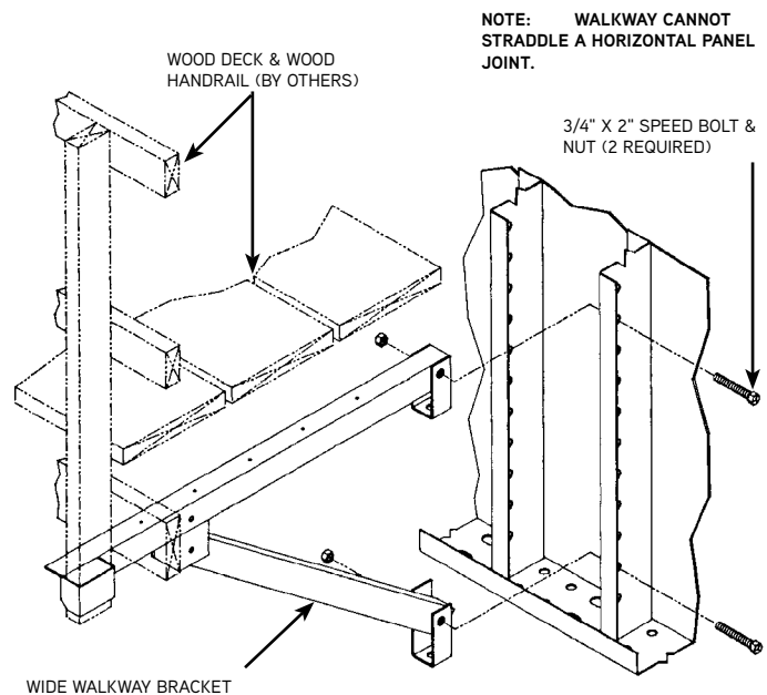
Wide Walkway Bracket Installation for Vertical Stiffeners
