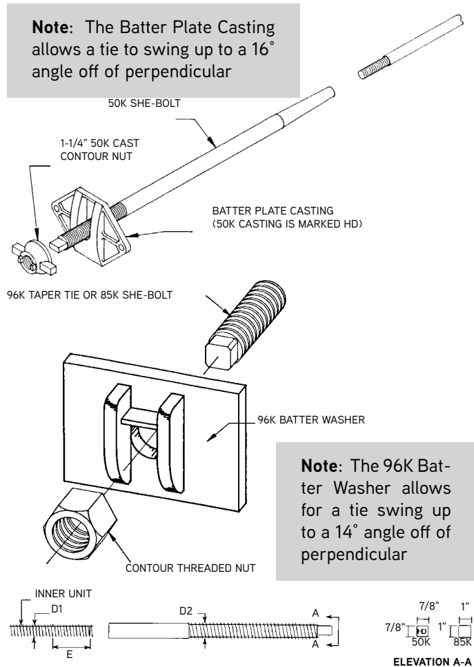
She-Bolt Capacities and Thread Dimensions
