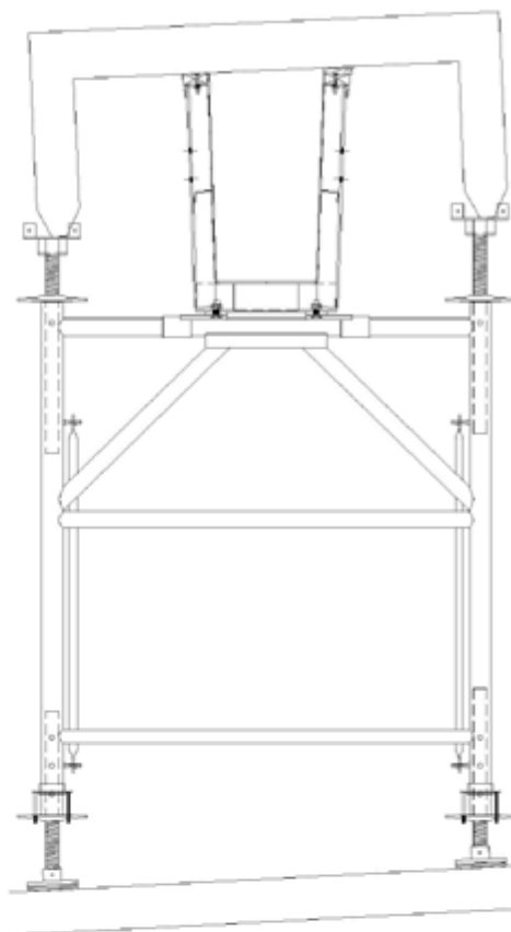
Ramped Slab Condition
