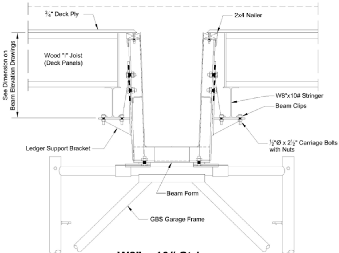
W8" x 10# Stringer to Ledger Bracket Attachment
