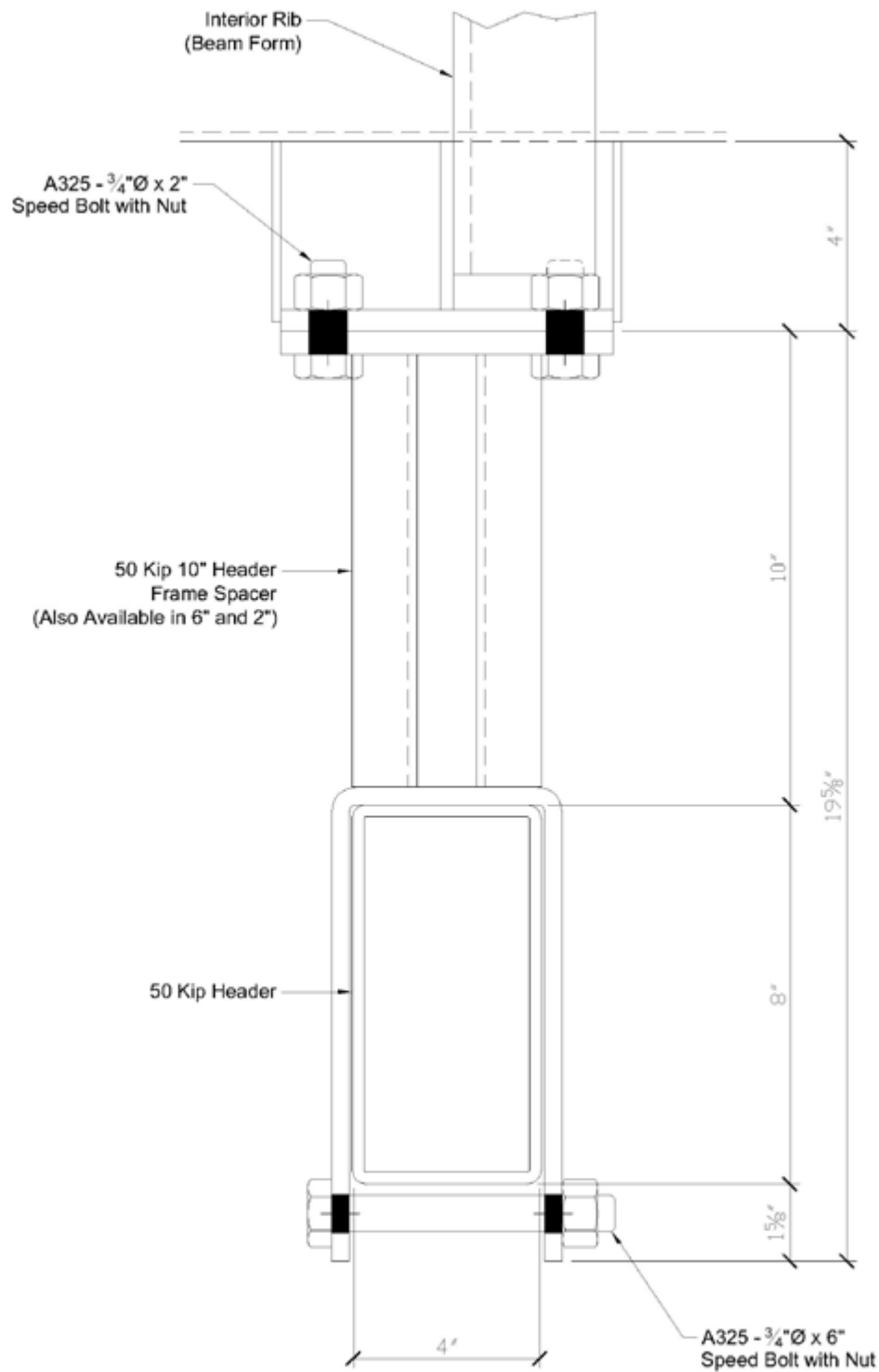
Beam Form to 50 Kip Header Bolt-Up Detail Using 50 Kip Frame Spacer
