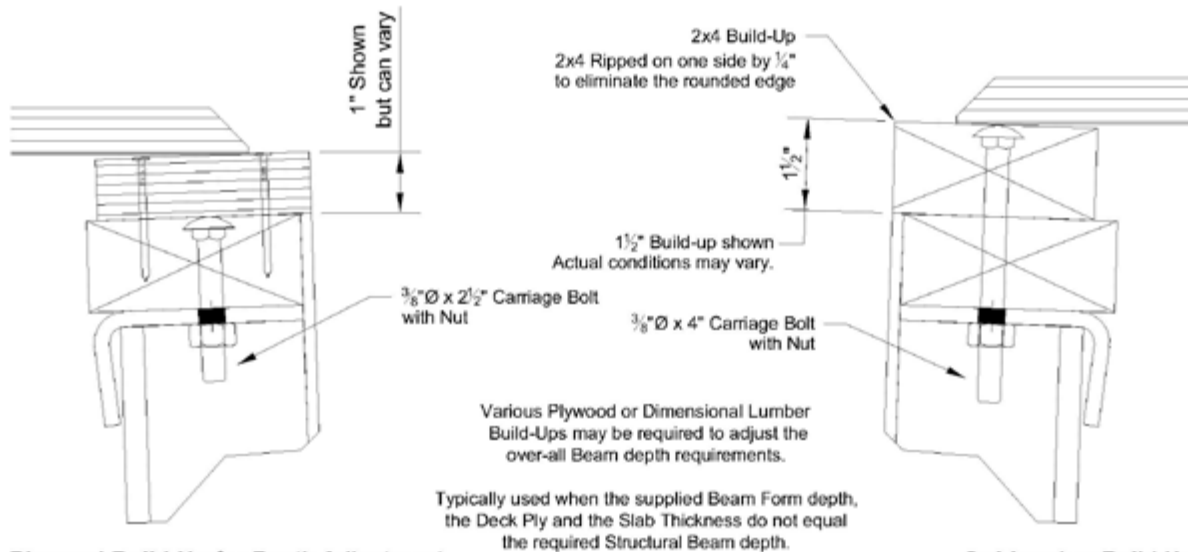
Plywood Build-Up for Depth Adjustment
