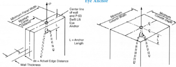
P53 Swift Lift Eye Anchor
